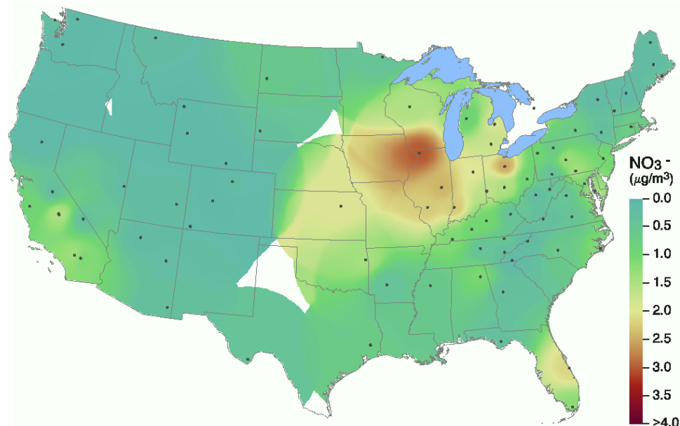
Figure 2-87. Annual average gas-phase \text{NO}_3 concentrations, 2004–2006. White areas on the map are areas where monitoring sites are absent and no information is available.
