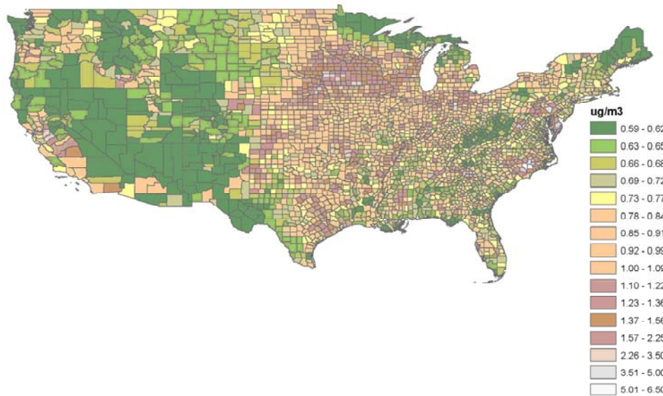
Figure 2-90. Estimated county-scale ambient NH 3 concentrations.
