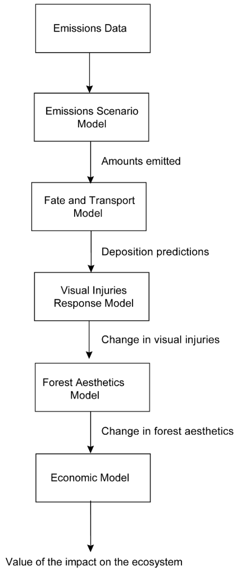
Figure F-5. Linkages from emissions to forest aesthetics.
