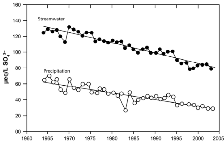
Figure A-3. Long-term record of SO 4 2- concentration in streamwater and precipitation at Watershed 6 of HBEF.
