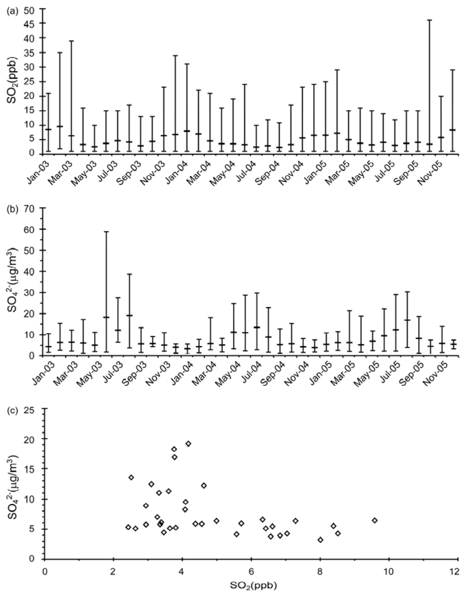
Figure 2-104. Philadelphia, 2003–2005. (a) Monthly mean, minimum, and maximum SO 2 concentrations. (b) Monthly mean, minimum, and maximum SO 4 2- concentrations. (c) Monthly mean SO 4 2- concentrations as a function of SO 2 concentrations.
