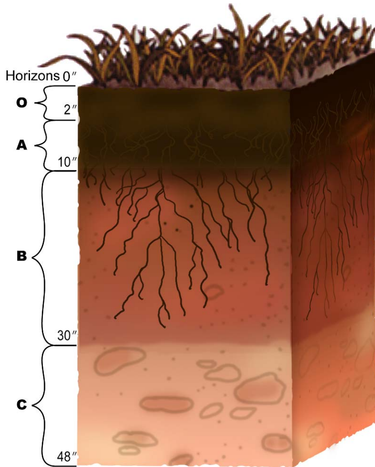
Figure 3-2. Diagram illustrates soil horizons commonly found. Each main horizon is denoted by a capital letter O ) Organic matter: Litter layer of plant residues in relatively undecomposed form. A ) Surface soil: Layer of mineral soil with most organic matter accumulation and soil life. This layer is depleted of iron, clay, aluminum, organic compounds, and other soluble constituents. B ) Subsoil: This layer accumulates iron, clay, aluminum and organic compounds. C ) Substratum: Layer of unconsolidated soil parent material. This layer may accumulate the more soluble compounds that bypass the “B” horizon.
