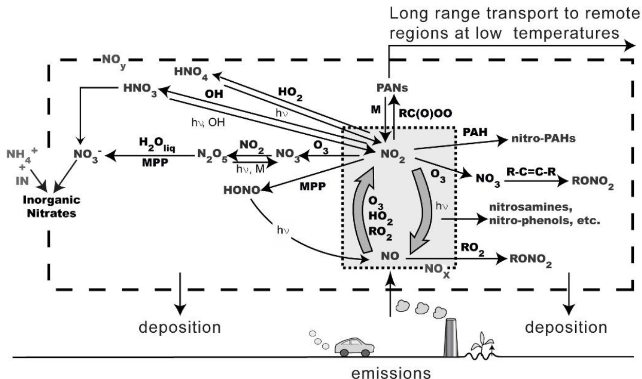
Figure 2-16. Atmospheric cycle of reactive oxidized N species. \text{NO}_y refers to all the species shown within the inner and outer box: \text{NO}_x to NO and \text{NO}_2 (in the inner box), and \text{NO}_2 to all the species outside of the inner box. IN refers to inorganic particulate species (e.g., sodium [\text{Na}^+] , calcium [\text{Ca}^{2+}] ), MPP to multiphase processes, h\nu to a solar photon, and R to an organic radical. Particle-phase \text{RONO}_2 are formed from the species shown on the right side. For the purposes of this document, “ \text{NO}_x ” is defined as the group of all N-containing compounds inside the large dashed-line box, the same group generally termed “ \text{NO}_y ” by atmospheric scientists.
