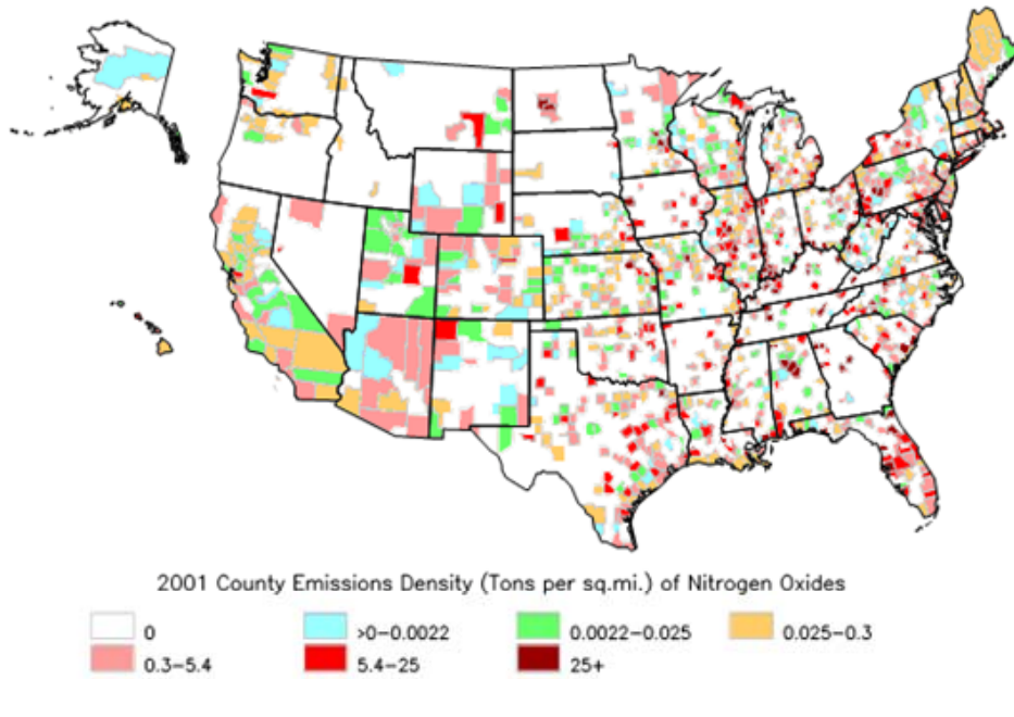
Figure 2-3. 2001 county-level total U.S. NO x (NO and NO 2 ) emissions densities (tons per square mile) from electric-generating utilities (EGUs). 1
