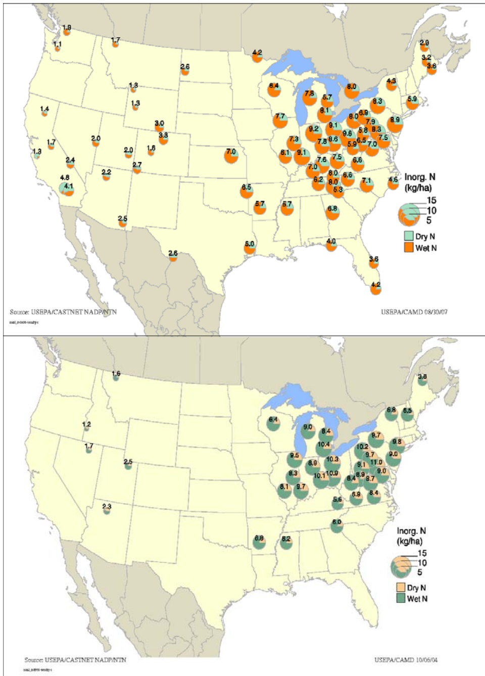
Figure 2-117. Total average yearly wet and dry inorganic N deposition, excepting NH 3 , for 2004–2006 (top) and 1989–1991 (bottom).
