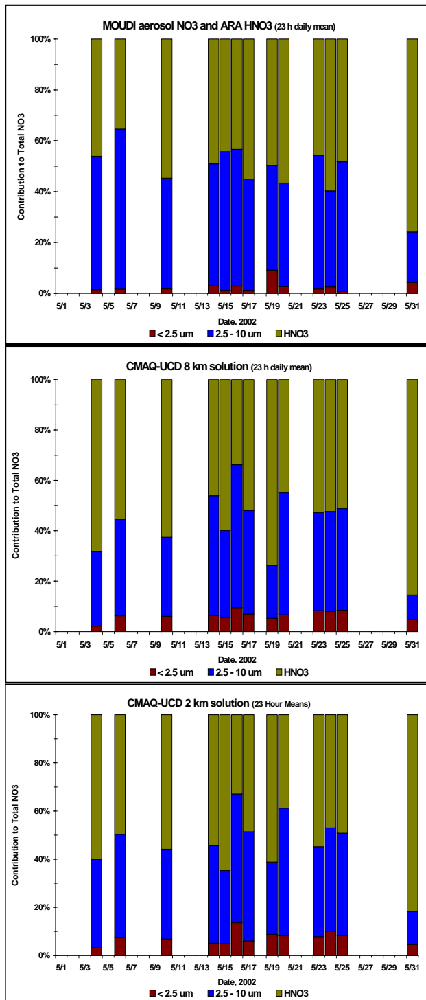
Figure 2-39. CMAQ-UCD predicted fractions and totals of total NO 3 for days in May 2002 with measurements in Tampa Bay, FL. Legend: red bars = <2.5 μm; blue bars = 2.5–10 μm; green bars = HNO 3 . Measured concentrations (top panel), CMAQ-UCD 8 km solution (middle panel) and CMAQ-UCD 2 km solution (bottom panel).
