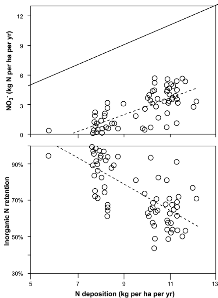
Figure 3-31. a) N export in stream water as a function of N deposition at the base of sampled watersheds. N export is represented by the equation \text{N}_{\text{exp}} = 0.85 \text{N}_{\text{dep}} - 5.8 ; r^2 = 0.56 ; p < 0.001 . (b) Watershed N retention decreases as N deposition at the base of the watersheds increases ( \text{N retention} = -0.07 \text{N deposition} + 1.44 ; r^2 = 0.50 ).
