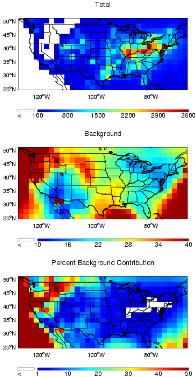
Figure 2-61. Annual mean concentrations of SO x deposition (SO 2 + pSO 4 ) (mg S/m 2 /yr) in surface air over the U.S. in the present-day (upper panel) and policy relevant background (middle panel) MOZART-2 simulations. The bottom panel shows the percentage contribution of the background to the present-day concentrations.
