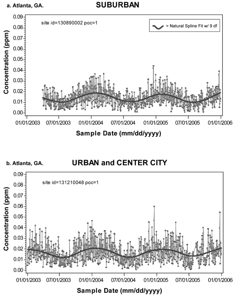
Figure 2-73. Time series of 24-h average NO 2 concentrations at individual monitoring sites in Atlanta, GA from 2003 through 2005. A natural spline function (with 9 degrees of freedom) was fit and overlaid to the data (dark solid line).
