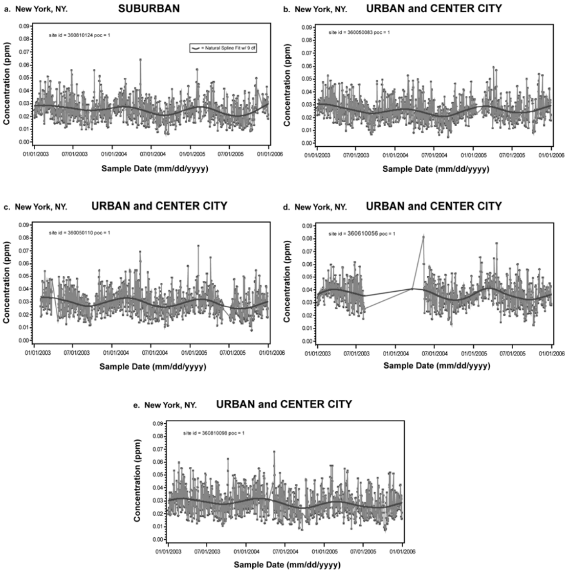
Figure 2-74. Time series of 24-h average NO 2 concentrations at individual monitoring sites in New York City from 2003 through 2005. A natural spline function (with 9 degrees of freedom) was fit and overlaid to the data (dark solid line).
