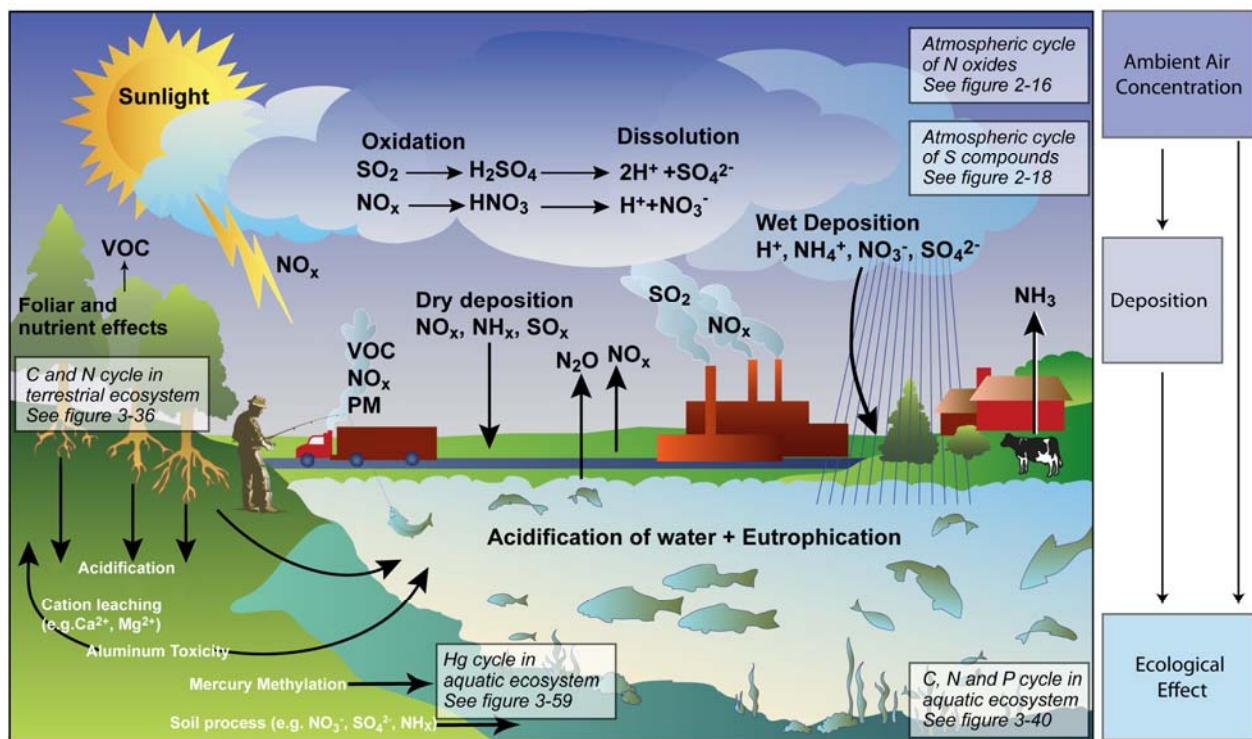
Figure 1-1. Biogeochemical cycles of NO x and SO x .
