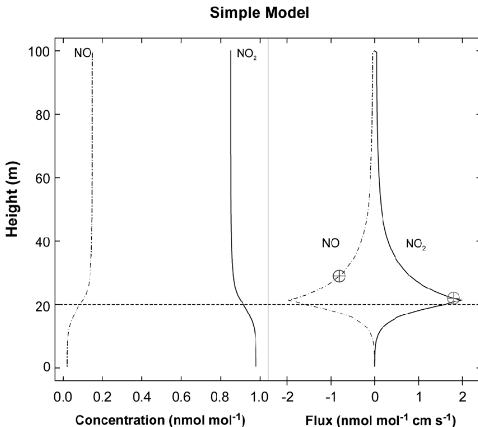
Figure 2-122. Simple NO x photochemical canopy model outputs. Left panel, concentrations of NO (dashed) and NO 2 (solid); right, fluxes of NO (dashed) and NO 2 (solid). Symbols indicate measurement heights for NO (29 m) and NO 2 (22 m) at Harvard Forest. The model solves the continuity equation for NO concentration at 200 levels, d/dz(-Kc[dNO/dz]) = PNO - LNO , where PNO = [NO]/t_1 , LNO = [NO]/t_2 , and zero net deposition or emission of NO x is allowed. NO x (NO + NO 2 ) is normalized to 1 ppb. t_1 = 70 s in this example. Due to the measurement height difference, observed upward NO 2 flux due to photochemical cycling alone should be substantially larger than observed downward NO flux attributable to the same process.
