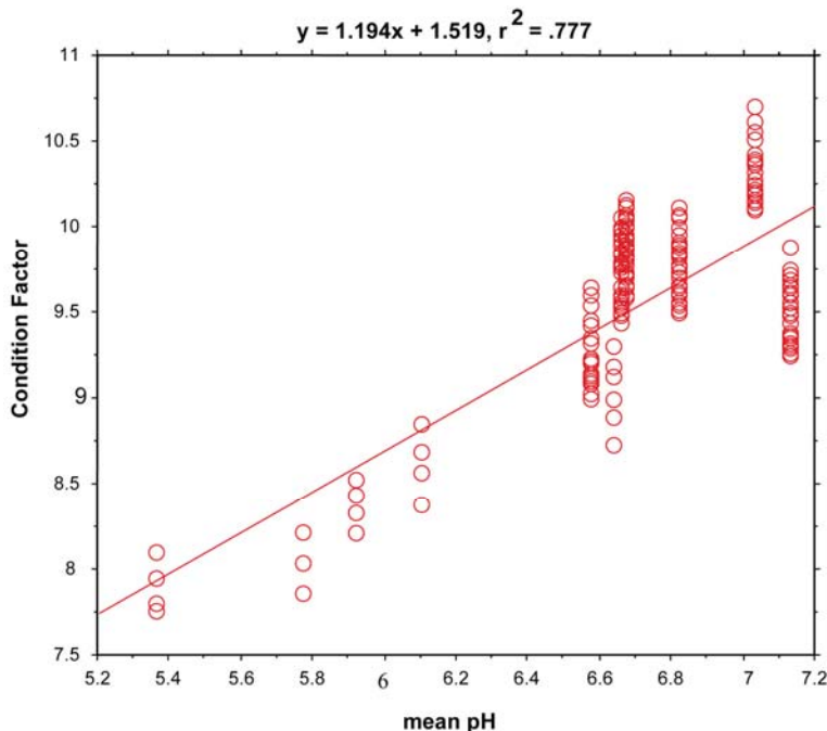
Figure 3-26. Length-adjusted condition factor (K), a measure of body size in blacknose dace ( Rhinichthys atratulus ) compared with mean stream pH among 11 populations (n = 442) in Shenandoah National Park. Values of pH are means based on quarterly measurements, 1991–1994; K was measured in 1994. The regression analysis showed a highly significant relationship (p < 0.0001) between mean stream pH and body size, such that fish from acidified streams were less robust than fish from circumneutral streams.
