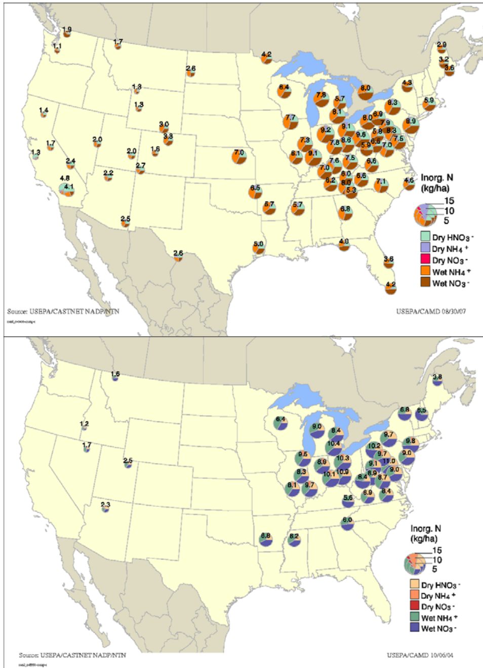
Figure 2-118. Total average yearly inorganic N deposition by species, excepting NH 3 , for 2004–2006 (top) and 1989–1991 (bottom).
