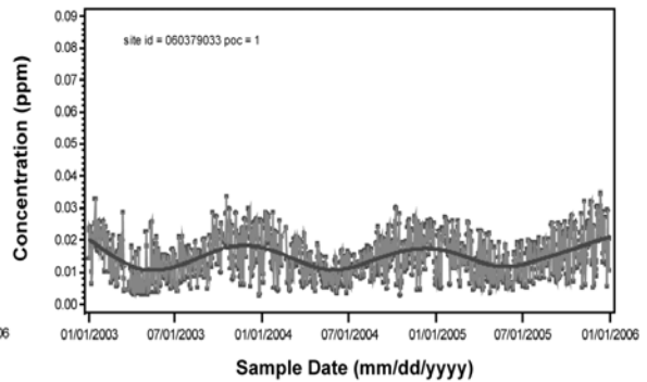
Figure 2-79. Time series of 24-h average NO 2 concentrations at individual monitoring sites in Los Angeles, CA from 2003 through 2005. A natural spline function (with 9 degrees of freedom) was fit and overlaid to the data (dark solid line).
