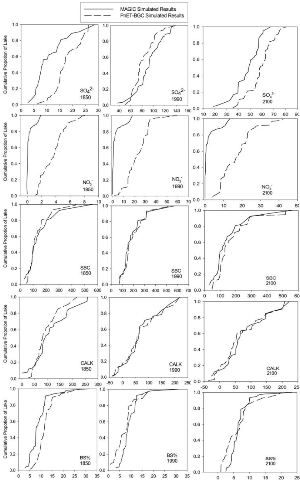
Figure 3-21. Cumulative distribution functions of selected major ions ( \mu\text{eq/L} ), calculated ANC of lakewater ( \mu\text{eq/L} ), and B horizon soil % base saturation for the MAGIC and PnET-BGC models. Results are shown for 1850, 1990, and 2100.
