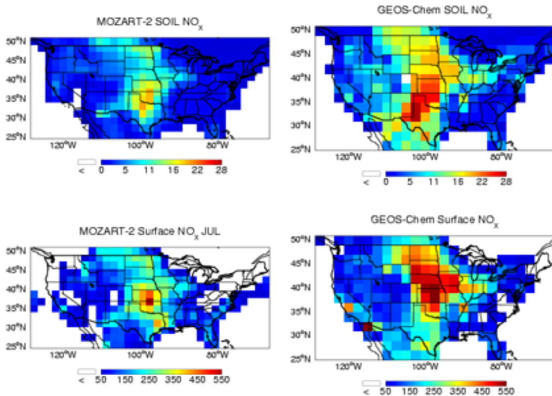
Figure 2-62. July mean soil NO emissions (upper panels; 1 \times 10^9 molecules/cm 2 /s) and surface PRB NO x concentrations (lower panels; ppt) over the U.S. from MOZART-2 (left) and GEOS-Chem (right) model simulations in which anthropogenic O 3 precursor emissions were set to zero in North America.
