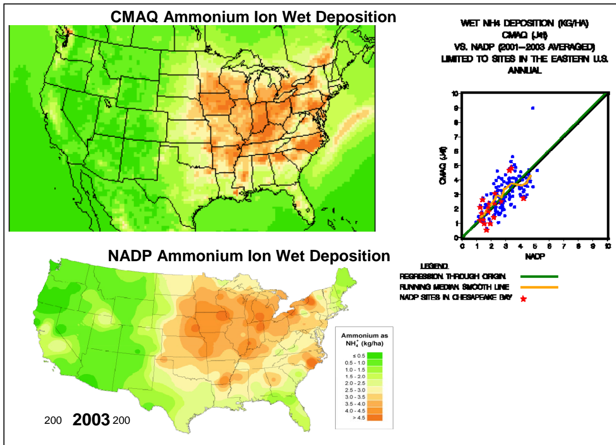
Figure 2-52. Comparison of CMAQ-predicted and NADP-measured \text{NH}_4^+ wet deposition. (top left) CMAQ prediction; (bottom left) NADP-measurements; (right) regression and smoothed median line through CMAQ predictions and NADP measurements with sites in the Chesapeake Bay watershed highlighted.
