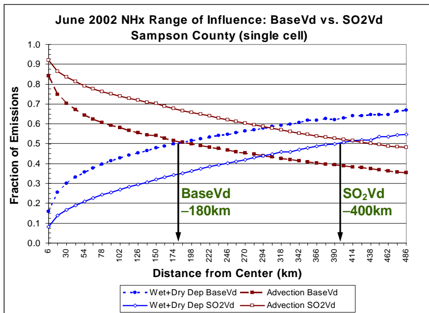
Figure 2-56. Range of influence (where 50% of emitted \text{NH}_3 deposits) from the high concentration Sampson County, NC, cell in the June 2002 CMAQ simulation of V_d sensitivities. Base case and sensitivity case total deposition (blue symbols and lines); base case and sensitivity case advection totals (red symbols and lines).
