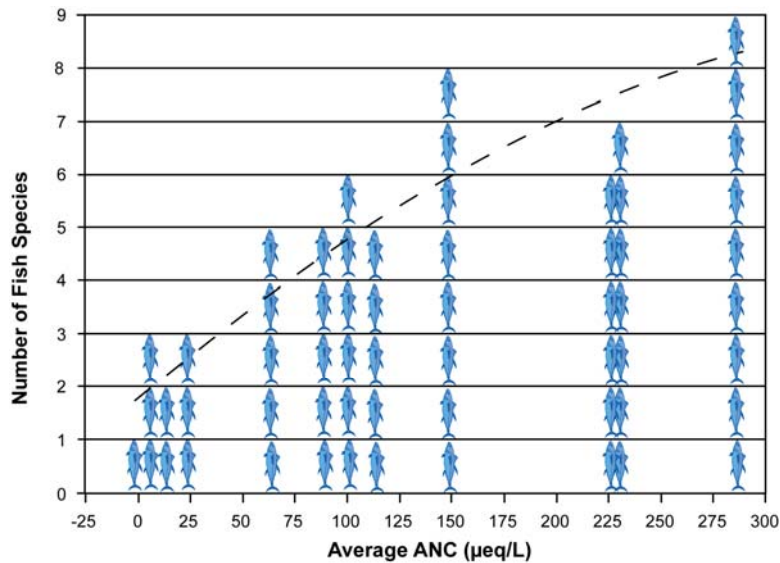
Figure B-18. Number of fish species among 13 streams in Shenandoah National Park. Values of ANC are means based on quarterly measurements, 1987–94. The regression analysis showed a highly significant relationship ( p < 0.0001 ) between mean stream ANC and number of fish species. Streams having ANC consistently < 75 \mu\text{eq/L} had three or fewer species.
