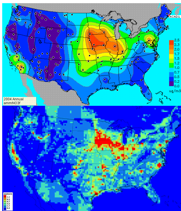
Figure 2-94. Maps of spatial patterns for average annual pNO_3 measurements (top), and for NH_3 emissions for April 2002 from the WRAP emissions inventory (bottom).
