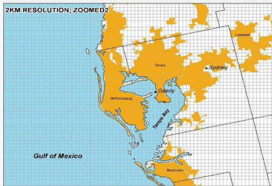
Figure 2-28. 2 km southeast U.S. CMAQ domain zoomed over Tampa Bay, FL.
