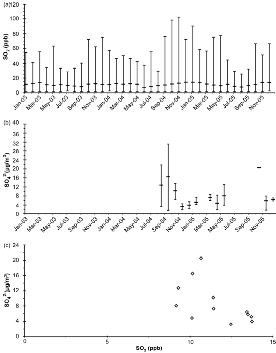
Figure 2-103. Steubenville, OH, 2003–2005. (a) Monthly mean, minimum, and maximum SO 2 concentrations. (b) Monthly mean, minimum, and maximum SO 4 2- concentrations. (c) Monthly mean SO 4 2- concentrations as a function of SO 2 concentrations.
