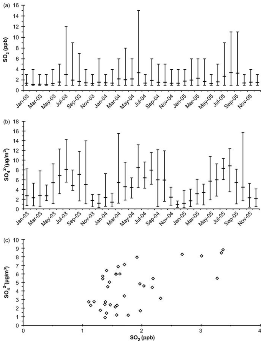
Figure 2-107. Phoenix, 2003–2005. (a) Monthly mean, minimum, and maximum SO 2 concentrations. (b) Monthly mean, minimum, and maximum SO 4 2- concentrations. (c) Monthly mean SO 4 2- concentrations as a function of SO 2 concentrations.
