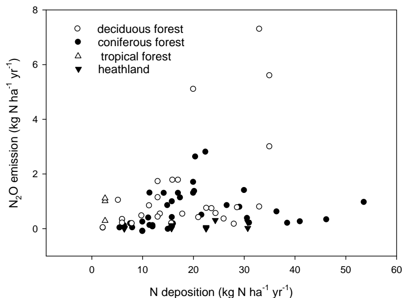
Figure 3-49. The relationship between \text{N}_2\text{O} emission and N deposition. The data were compiled from 36 independent studies.
