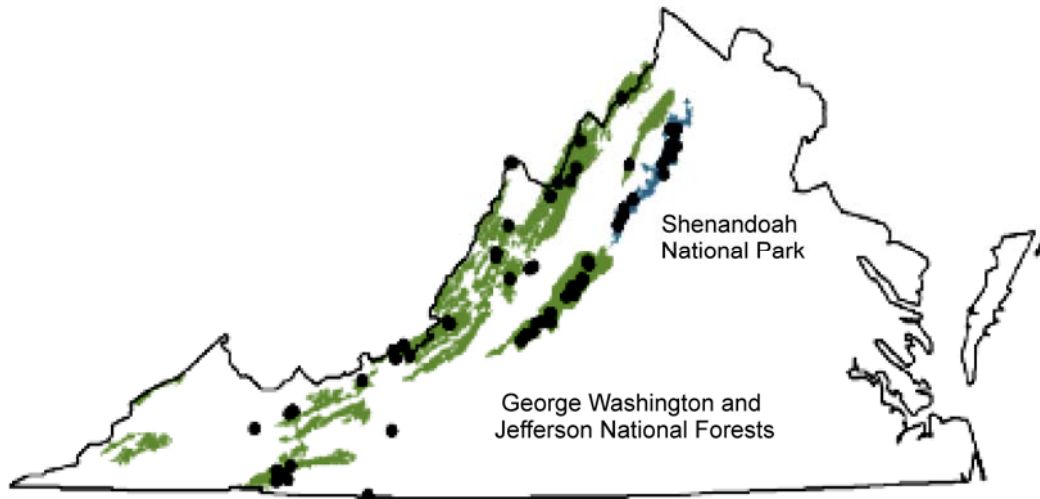
Figure A-5. SWAS-VTSS Program Study Sites. The length of the stream water chemical composition record for SWAS-VTSSS study watersheds is 20 to 28 years. SWAS sites are located in Shenandoah National Park (shaded blue). VTSSS sites are mainly located in Virginia's National Forests (shaded green).
