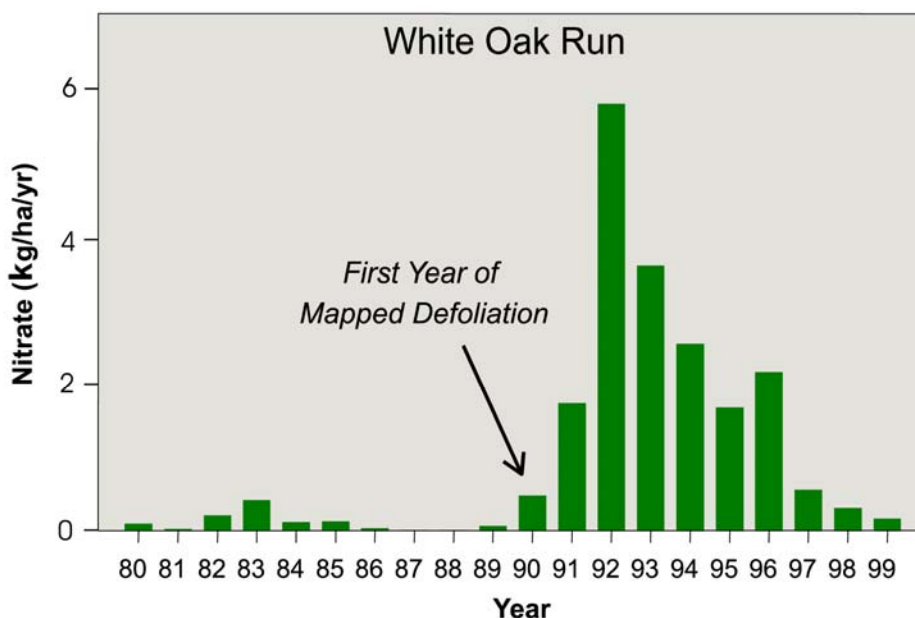
Figure C-6. Effect of watershed defoliation by the gypsy moth caterpillar on \text{NO}_3^- flux in streamwater. White Oak Run was heavily defoliated for three consecutive years. The watershed area defoliated was 46.5% in 1990, 92.9% in 1991, and 90.4% in 1992. In 1993, the gypsy moth population collapsed and there was no further defoliation.
