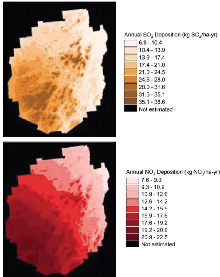
Figure 3-18. Spatial patterns in predicted wet SO 4 2- and NO 3 - deposition in the Adirondack Park during the period 1988 to 1999.
