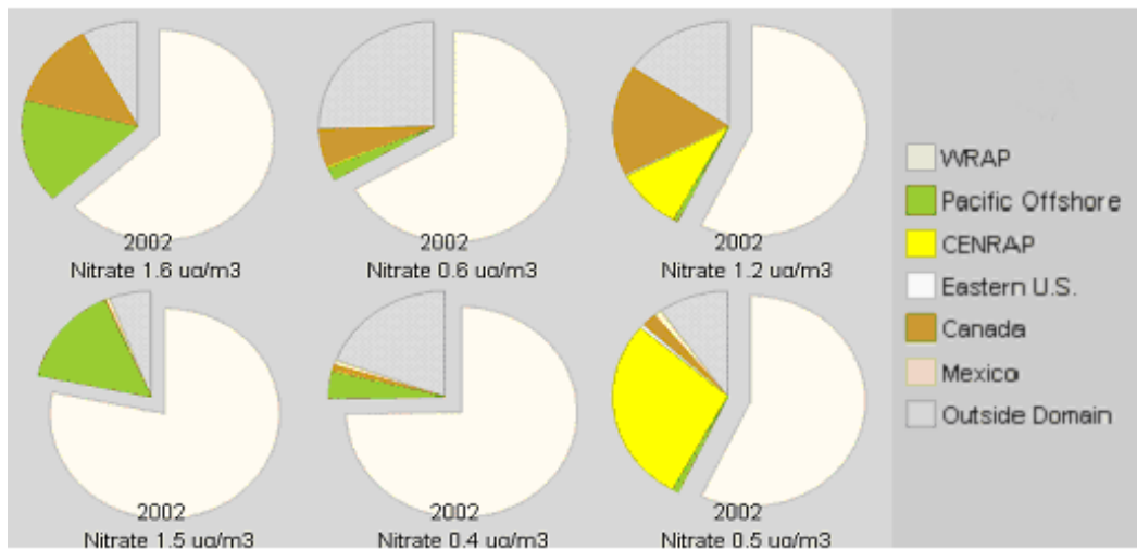
Figure 2-96. Particulate NO 3 source attribution by region using CAMx modeling for six western remote area monitoring sites. Top left to right Olympic NP, WA; Yellowstone NP, WY; Badlands NP, SD; bottom left to right San Geronio (W), CA; Grand Canyon NP, AZ; and Salt Creek (W), NM. WRAP includes North Dakota, South Dakota, Wyoming, Colorado, New Mexico and all states further west. CENRAP includes all states east of WRAP and west of the Mississippi River including Minnesota. Eastern U.S. includes all states east of CENRAP. The Pacific Offshore extends 300km to the west of California, Oregon, and Washington. Outside Domain refers to the modeling domain, which extend hundreds of kilometers into the Pacific and Atlantic Oceans and from Hudson Bay Canada to just north of Mexico City.
