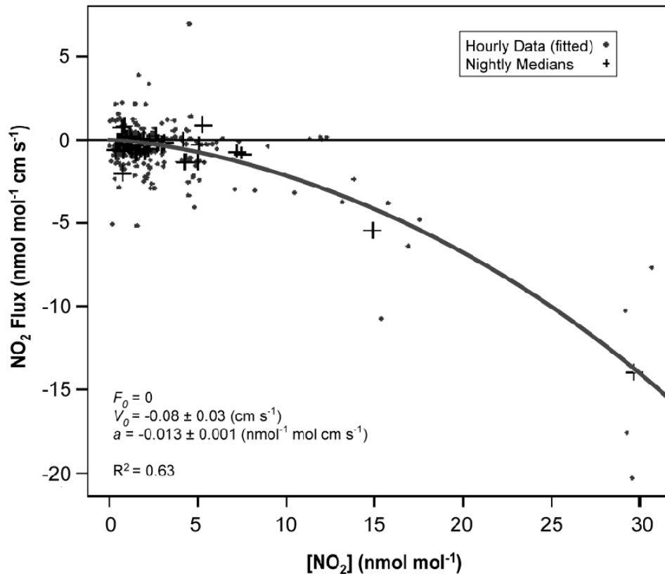
Figure 2-123. Hourly (dots) and median nightly (pluses) \text{NO}_2 flux vs. concentration, with results of least squares fit on the hourly data (curve).
