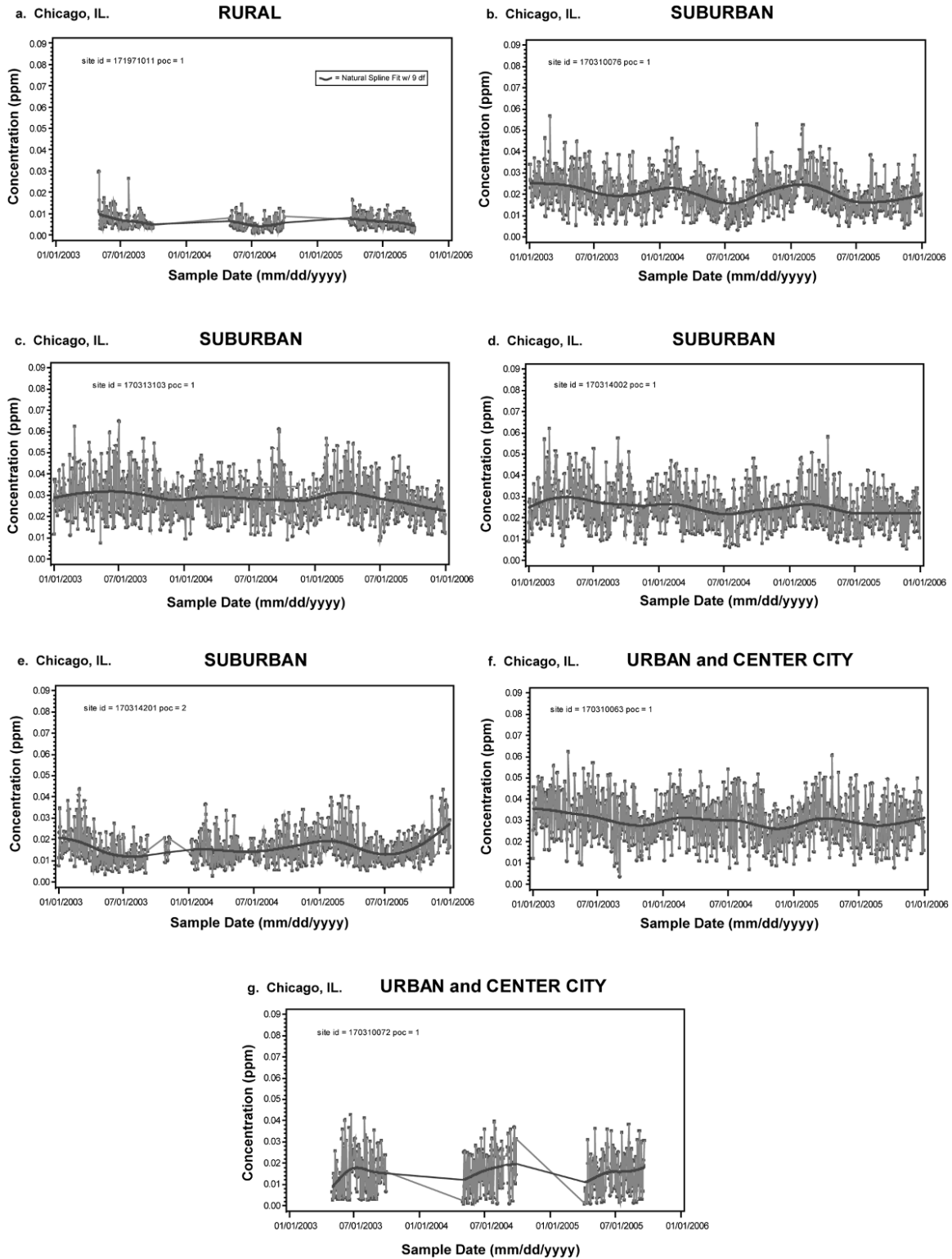
Figure 2-75. Time series of 24-h average NO 2 concentrations at individual monitoring sites in Chicago, IL from 2003 through 2005. A natural spline function (with 9 degrees of freedom) was fit and overlaid to the data (dark solid line).
