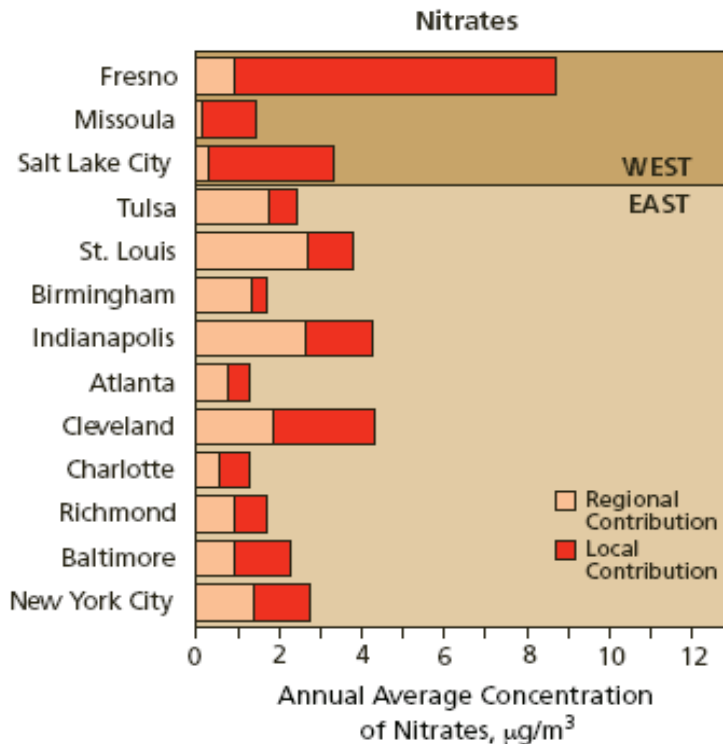
Figure 2-93. Regional and local contributions to annual average PM 2.5 by pNO 3 for select urban areas based on paired IMPROVE and CSN monitoring sites.
