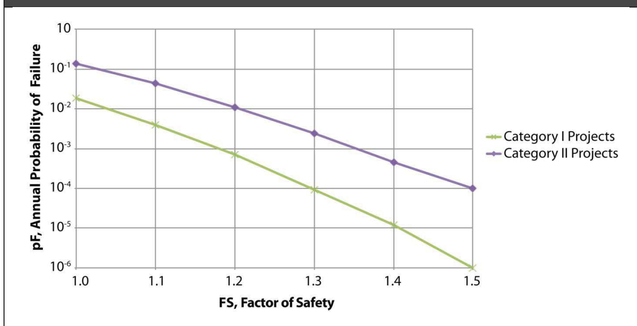
Figure 4-12. Annual Probability of Dam Failure vs. Factor of Safety (after Silva et al. 2008)
