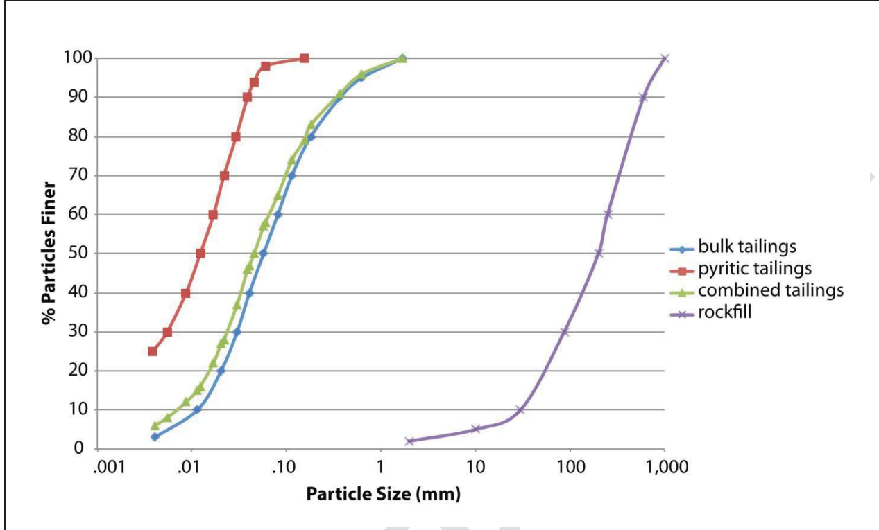
Figure 4-13. Representative Particle Size Distribution for Tailings Solids (Bulk and Cleaner or Pyritic Tailings) and Tailings Dam Rockfill
