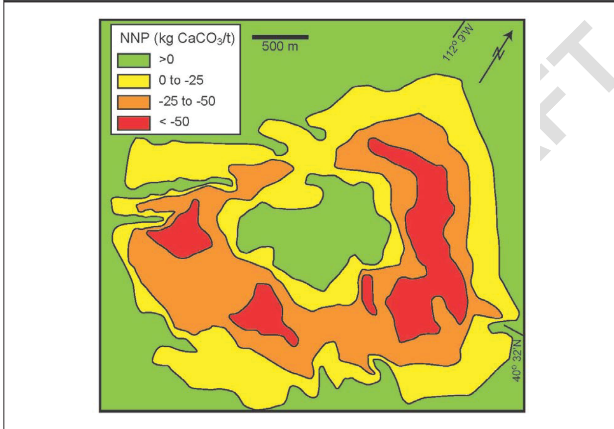
Figure 4-3. Plan View of the Distribution of Net Neutralizing Potential (NNP) Values at the Bingham Canyon Porphyry Copper Deposit, Utah. Bingham Canyon shares many geologic features with the Pebble deposit. NNP values greater than 0 are net alkaline; NNP values less than 0 are net acid. Modified from Borden (2003).
