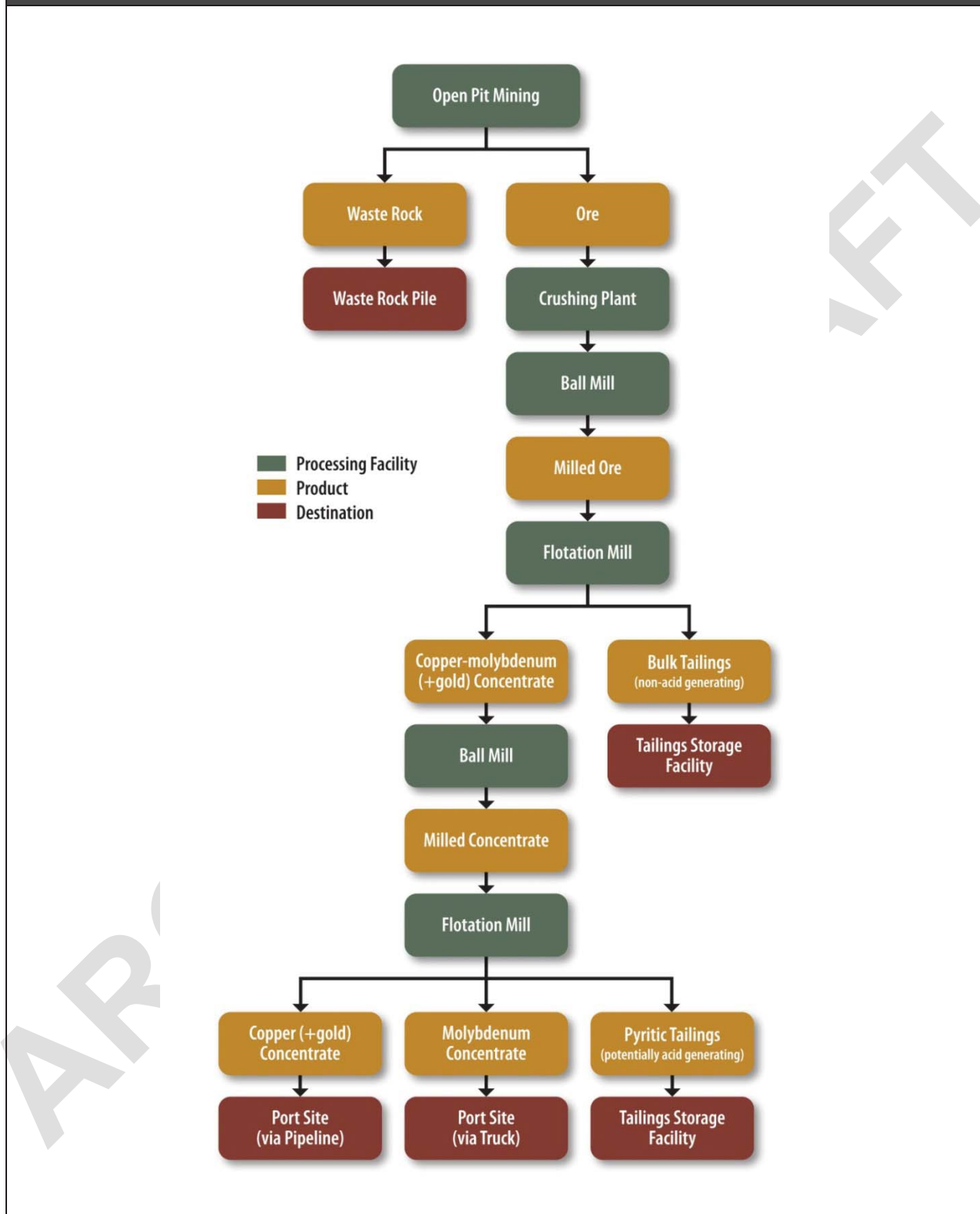
Figure 4-4. Simplified Schematic of Mined Material Processing
