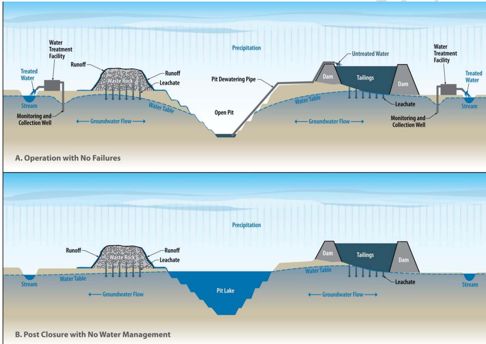
Figure 4-9. Simplified Schematic Illustrating Water Management and Movement at the Mine. Water movement and management is shown for two periods: A. routine operation, assuming no failures and B. post-closure, assuming no water management.
