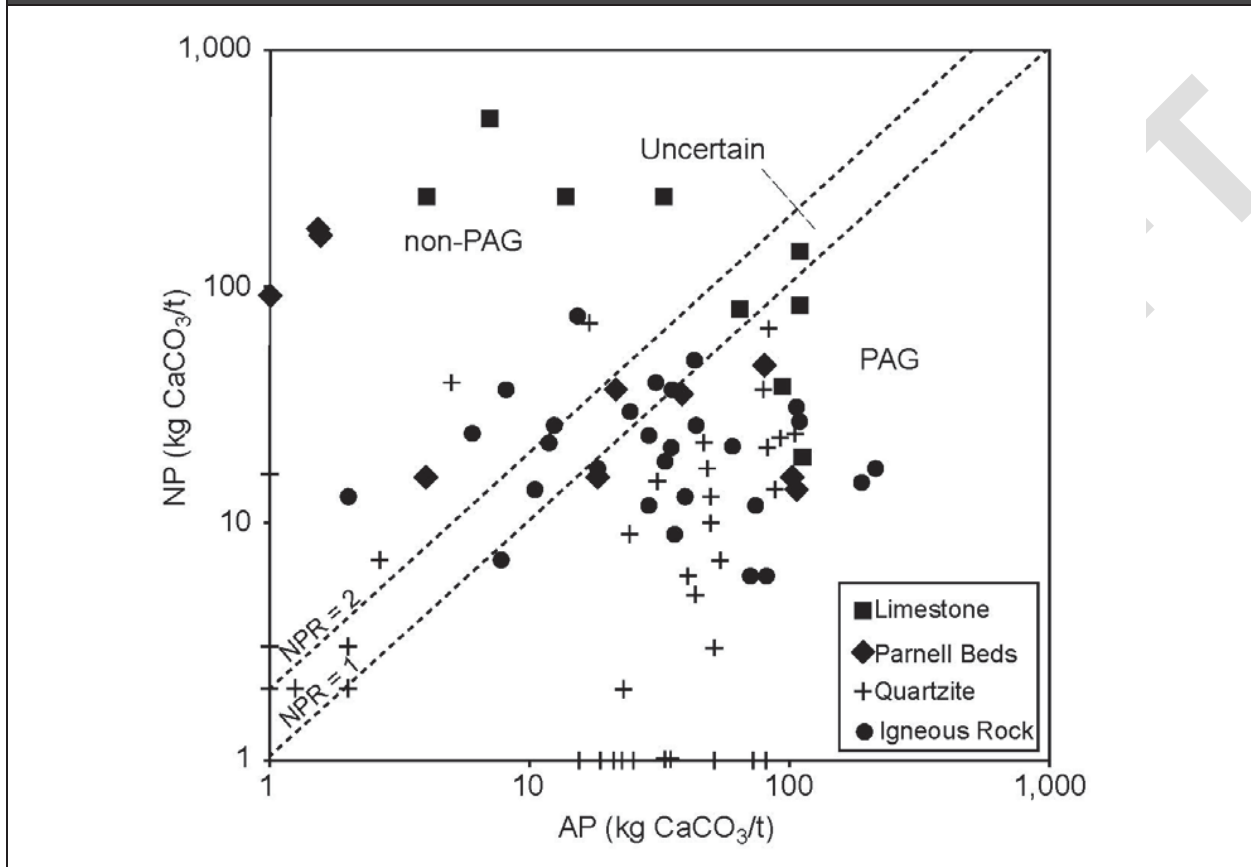
Figure 4-2. Plot of Neutralizing Potential (NP) vs. Acid-Generating Potential (AP) for Mineralized Rock Types at the Bingham Canyon Porphyry Copper Deposit, Utah. Bingham Canyon shares many geologic features with the Pebble deposit. Modified from Borden (2003).
