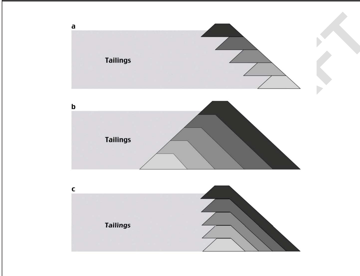
Figure 4-5. Cross-Sections Illustrating a) Upstream, b) Downstream, and c) Centerline Tailings Dam Construction. In each case, the initial dike is illustrated in light gray, with subsequent dike raises shown in darker shades (modified from Vick 1983). Tailings dams in our mine scenario are assumed to use the downstream construction method.
