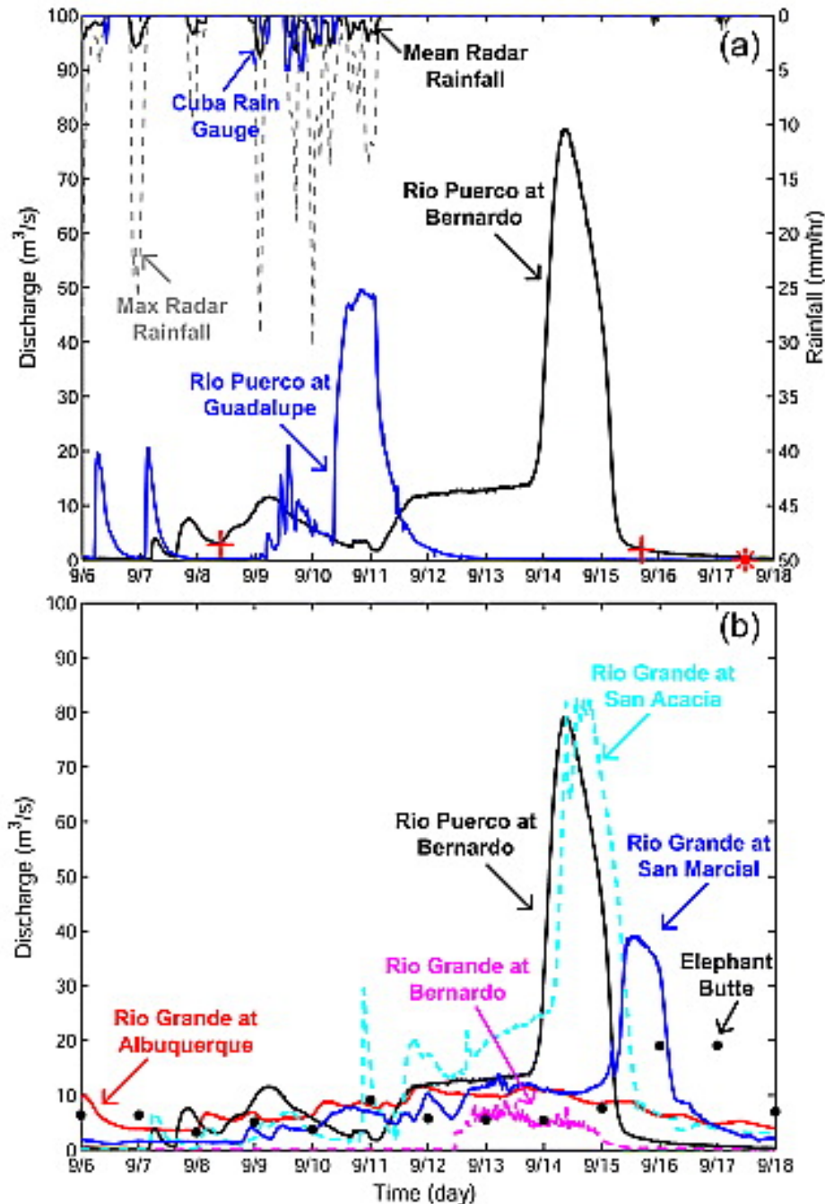
Figure 3-2. Time series of rainfall and streamflow observations in the Rio Puerco and Rio Grande, 6–18 September 2003. Source: Reprinted from Analysis of a monsoon flood event in an ephemeral tributary and its downstream hydrologic effects, (2006) by Vivoni et al. with permission of John Wiley & Sons.
